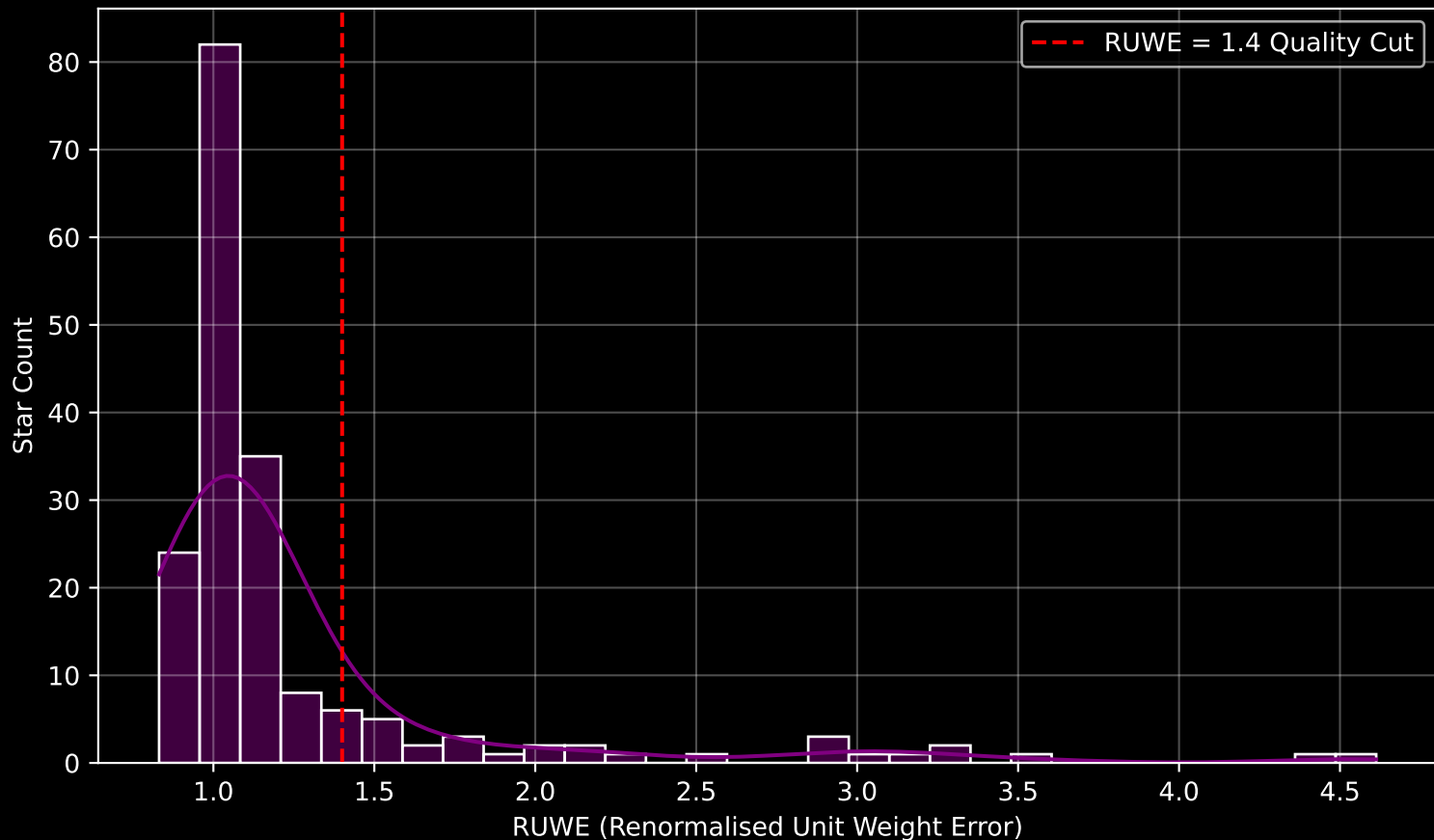
GAPOGEE DR17 Field [164+32_MGA] RUWE Distribution (n= 182)
