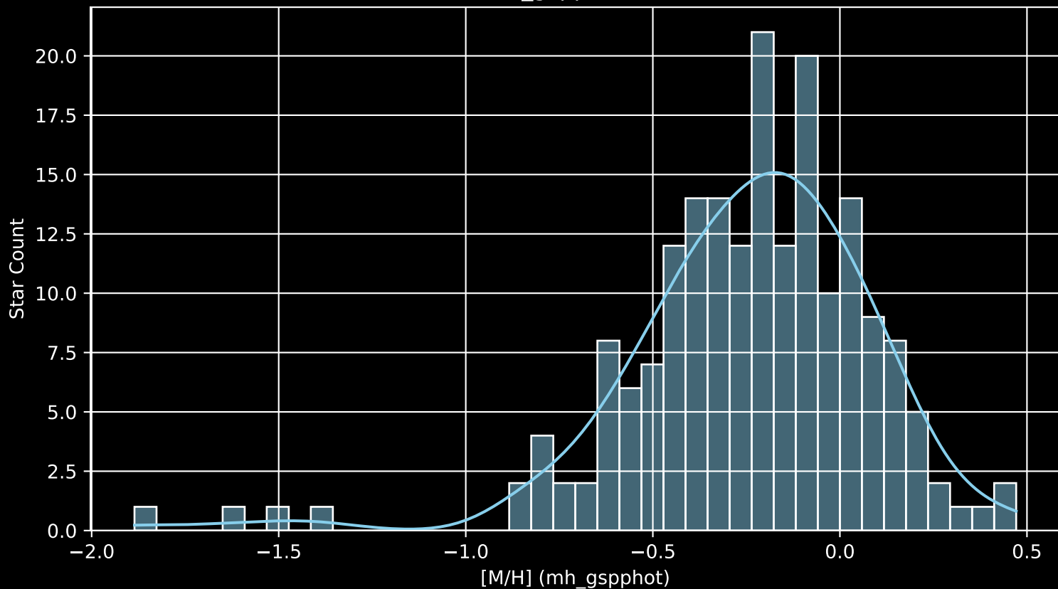
APOGEE DR17 Field: [164+32_MGA [M/H] (mh_gspphot) (n= 192)
