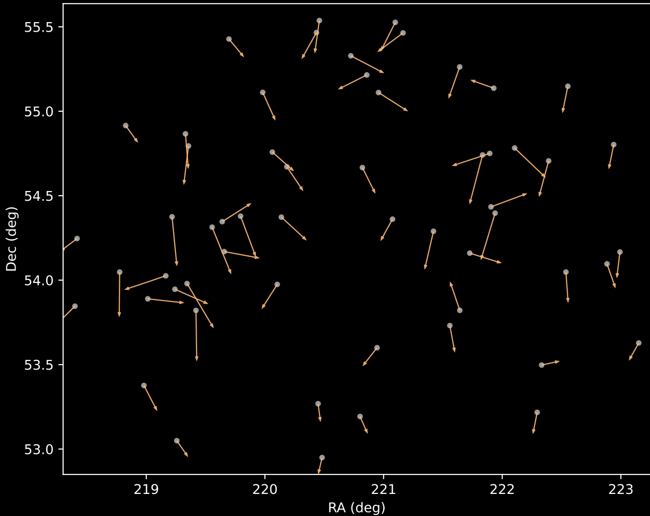
APOGEE DR17 Cluster 3 Proper Motion Vectors (n=57)
